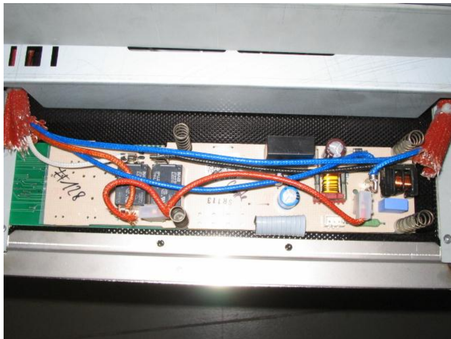
P29 ..EO3000 (alternate electronic unit)
