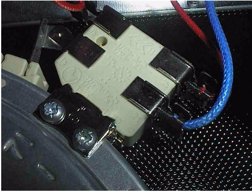
P29 ..EO3000 (alternate electronic unit)
