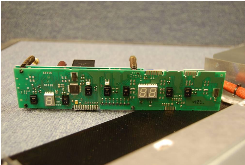
Control unit touch sensor and display PCB
