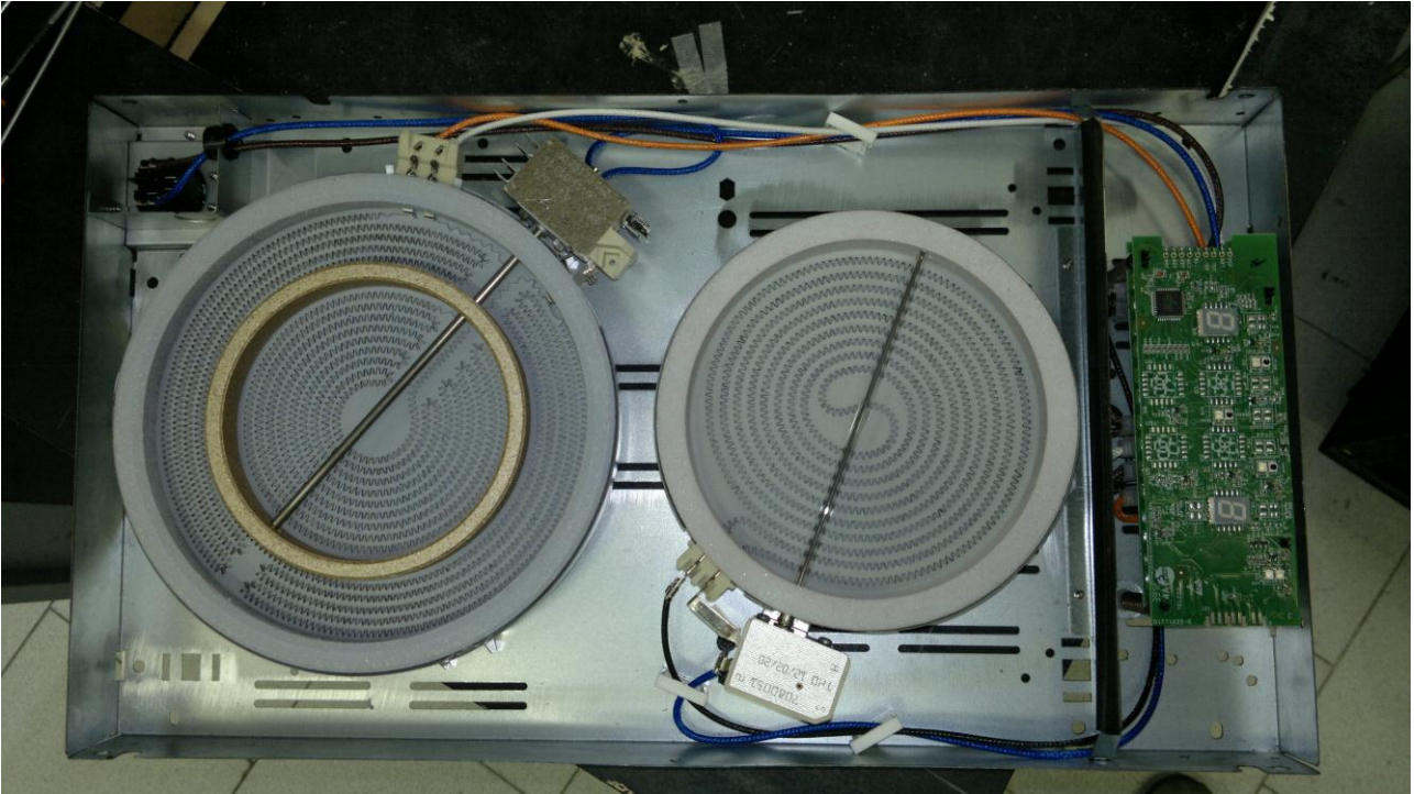
Hob with double zone
