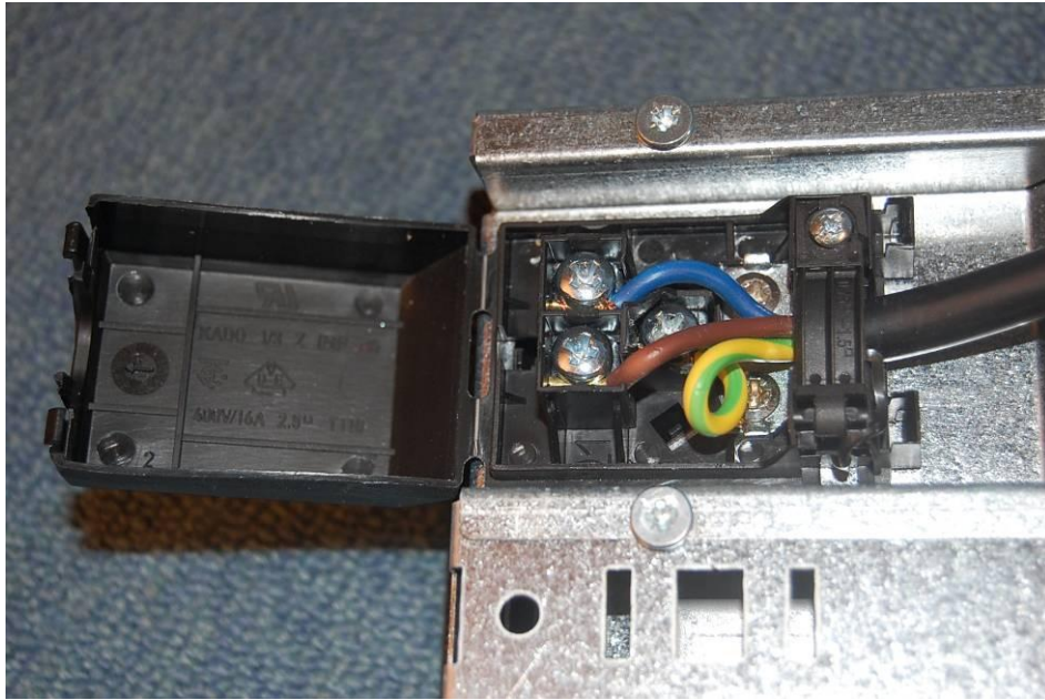
Supply terminal and cord anchorage
